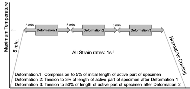
Figure 7: Treatment No. 1
