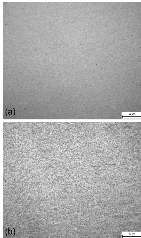
Figure 13: Microstructure of material 8 without annealing: a) without deformation, b) with 50 % deformation
