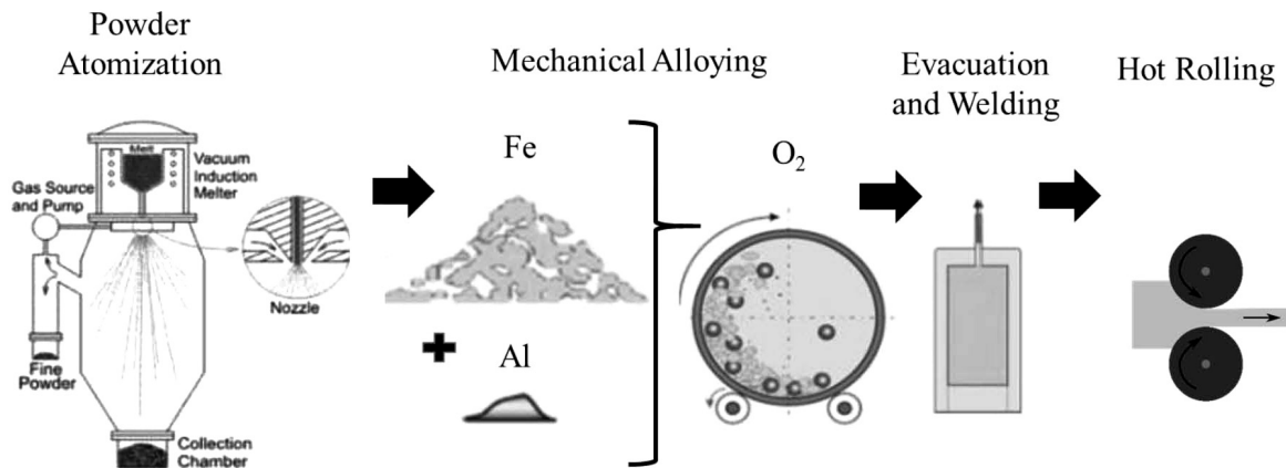
Figure 1: Material-preparation process
