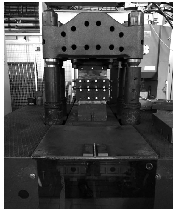
Figure 5: Hydraulic forging press
