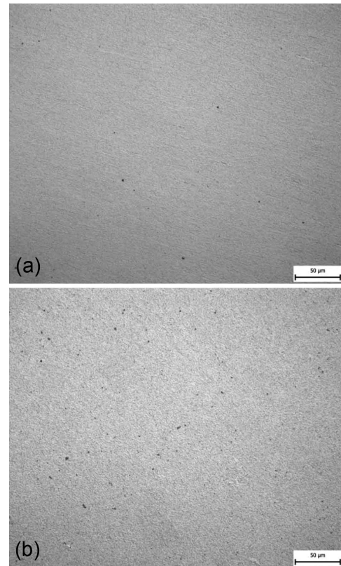
Figure 17: Microstructure for material 8 h with 20 h annealing: a) without deformation, b) with 50 % deformation
