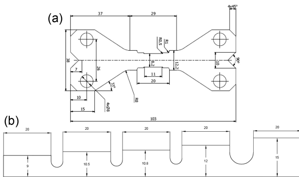
Figure 2: Specimen dimensions in mm: a) type 1, b) type 2
