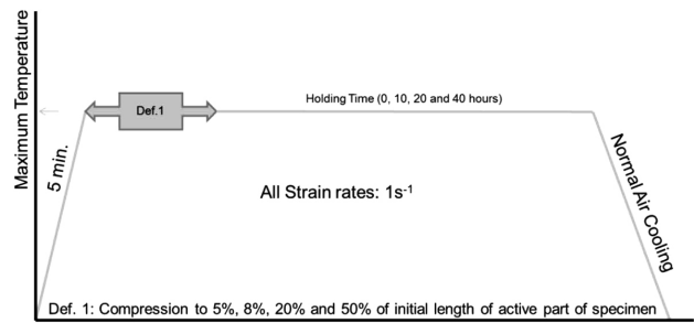
Figure 8: Treatment No. 2
