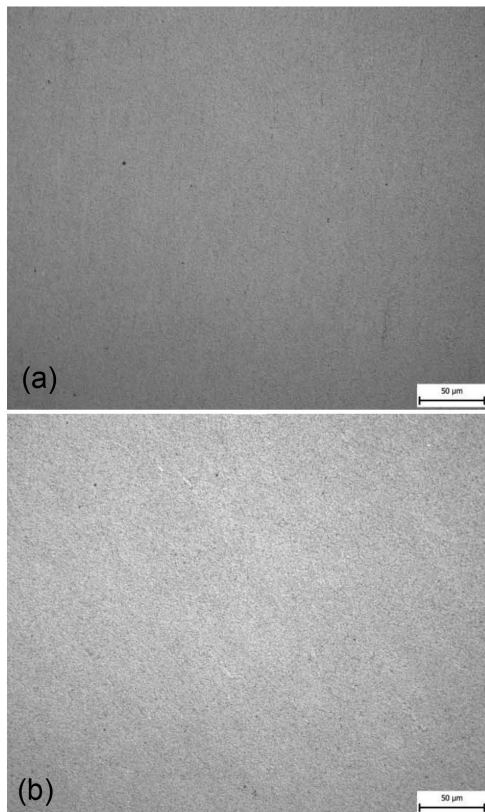
Figure 19: Microstructure for material 8 h with 40 h annealing: a) without deformation, b) with 50 % deformation
