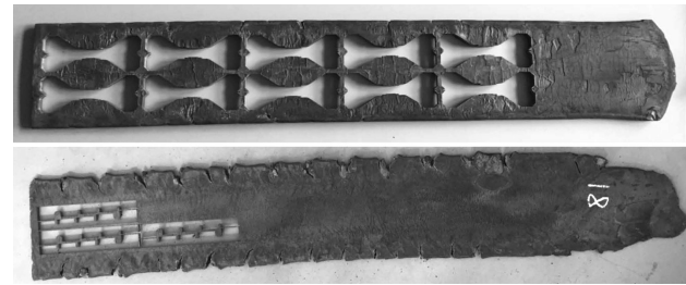
Figure 4: Positions of specimens on a rolled semi-product: a) type 1, b) type 2
