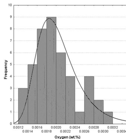
Figure 3: Oxygen content – forging
