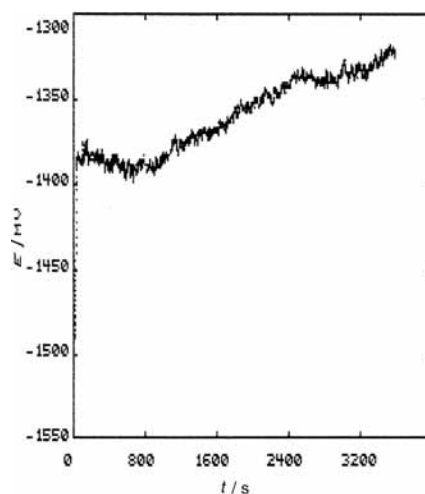
Figure 10: Corrosion potential vs. time for alloy 1 in 0.51 M NaCl
