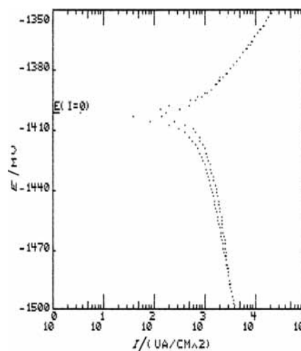
Figure 9: Potentiodynamic cathodic and anodic polarization curves for alloy 1 in 0.51 M NaCl. Scan rate 1 mV/s
