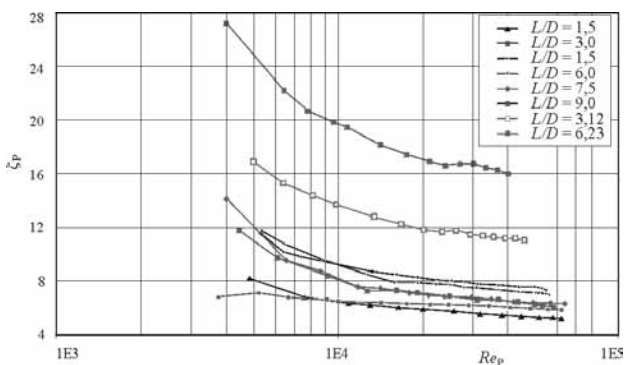
Figure 1: Dependence of the coefficient of the local resistance of the ceramic filters on the Reynolds number and the filter's slenderness Slika 1: Odvisnost koeficienta lokalnega upora keramičnega filtra od Reynoldsovega števila in od vitkosti filtra
